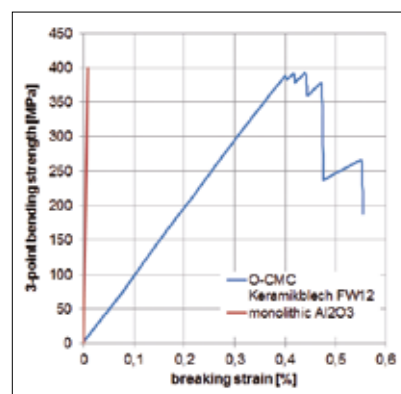
Fig. 2 Stress-strain curve of monolithic ceramic in comparison to O-CMC material
