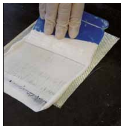
Fig. 3 Infiltration of ceramic fabric with matrix slurry for lamination process
