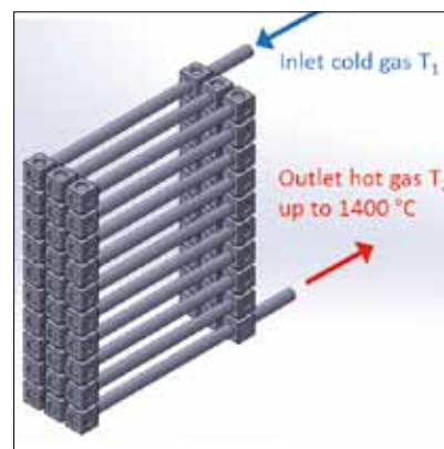
Fig. 9 Sketch of a high-temperature heat exchanger made of SSiC for the heat recovery at temperatures up to 1400 °C
