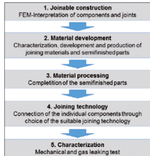
Fig. 11 Steps for the development of joining processes for ceramics and CMC
